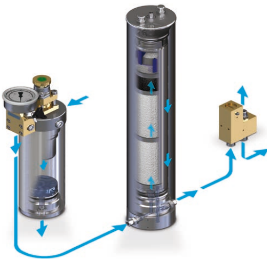
P41 Purification system
